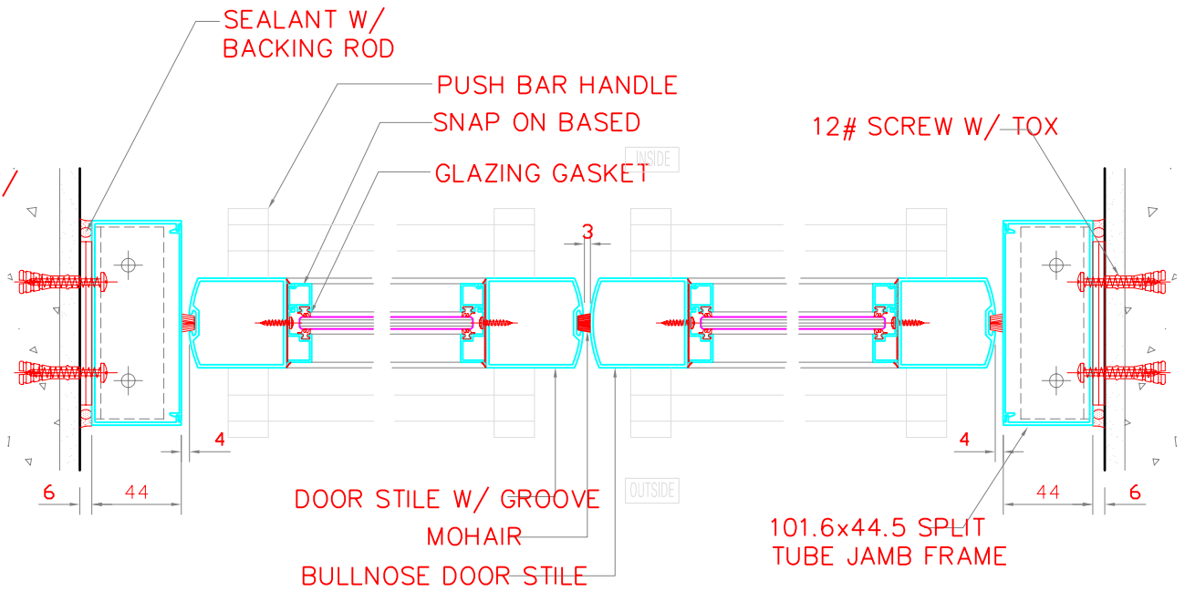
DETAIL-2
