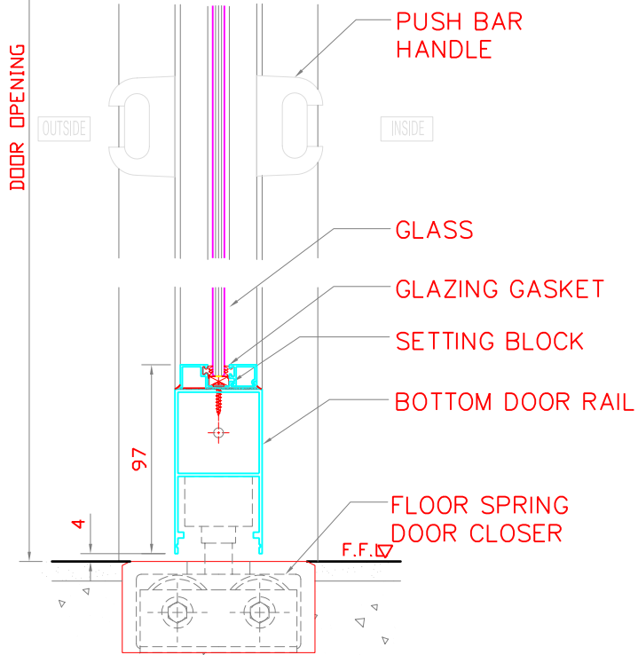
DETAIL-1
