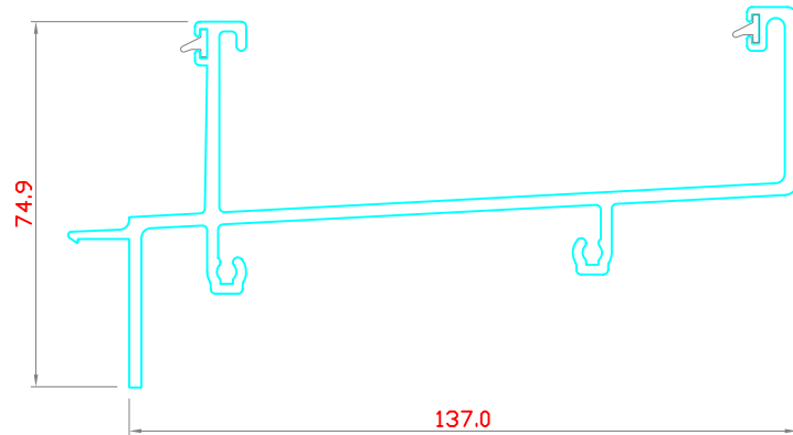
STACKHEAD FRAME 5000-SPS03
