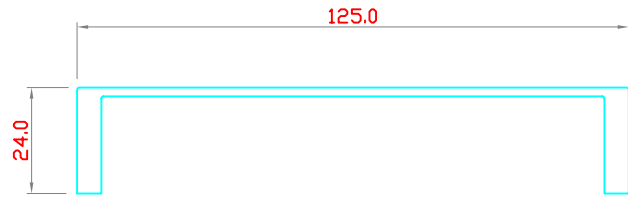
EXTENDED FEMALE MULLION 5000-SP2
