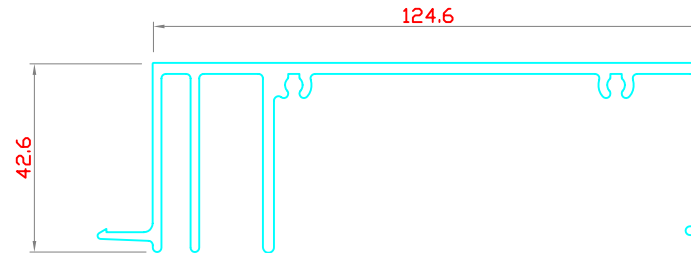
STACKSILL FRAME 5000-SPS01
