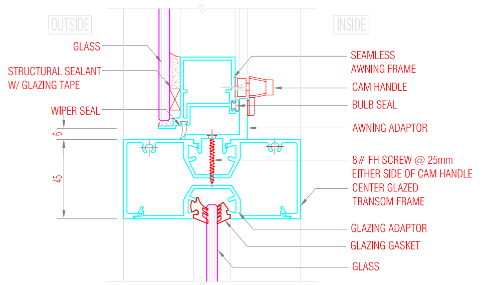
DETAIL-4
