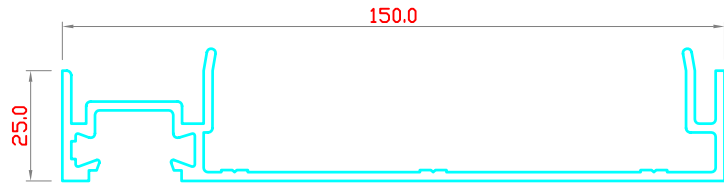
FORWARD GLAZED: FEMALE MULLION FRAME 5000-SP502
