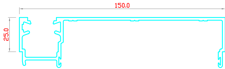
FORWARD GLAZED: MALE MULLION FRAME 5000-SP501
