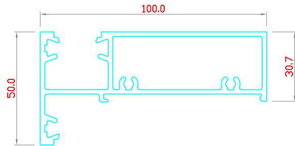
FORWARD GLAZED: HEAD/ SILL/ TRANSOM FRAME 5000-SP510
