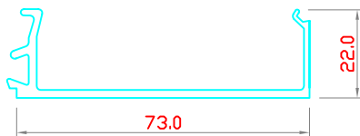
FORWARD GLAZED: GLAZING BEAD 5000-SP518
