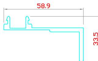
AWNING ADAPTOR 5000-SP521
